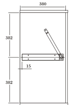
Bottom guide rail installation plan
